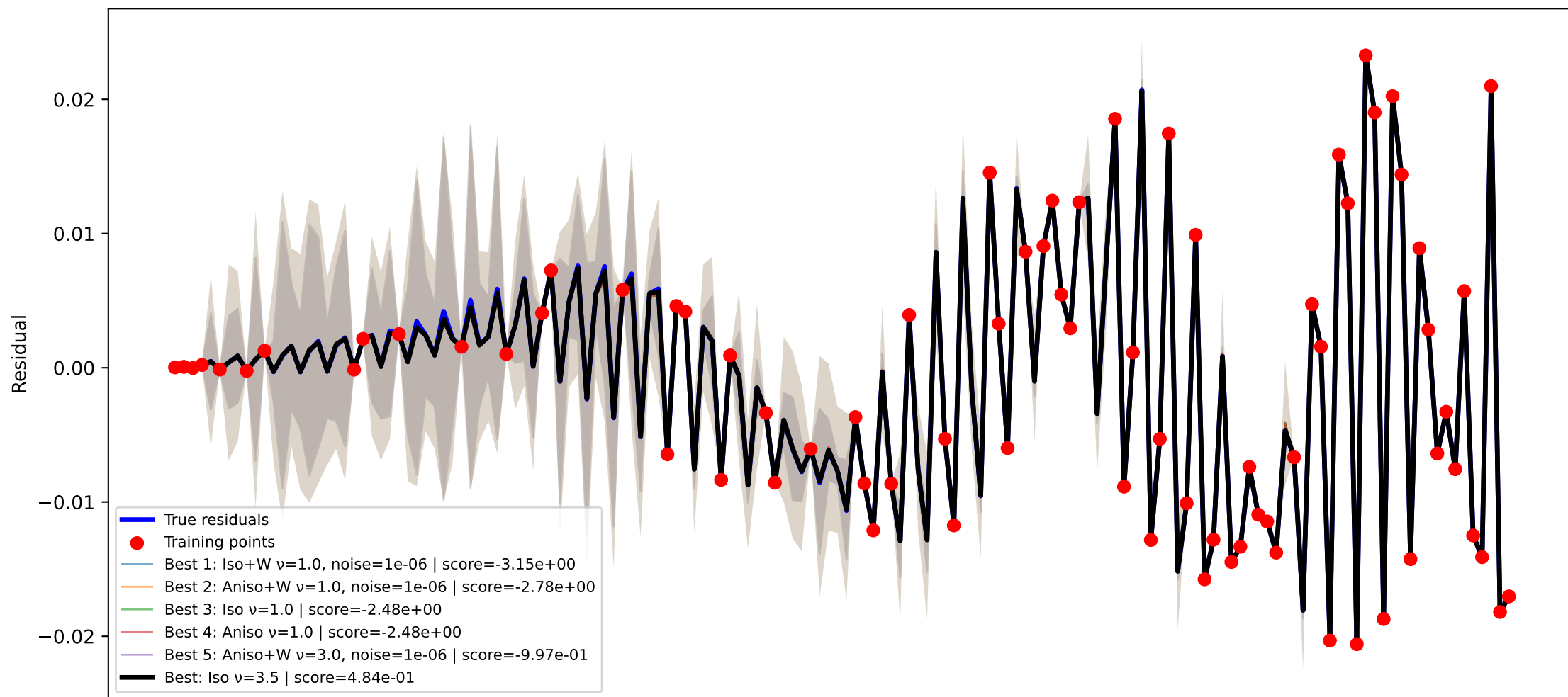
GPR kernel comparison node=36 RMSE=9.633e-05, train RMSE=1.184e-11
